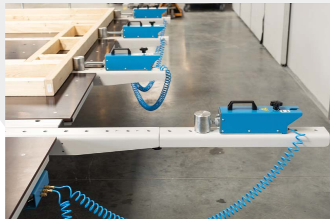
Removeable Beam Extensions
