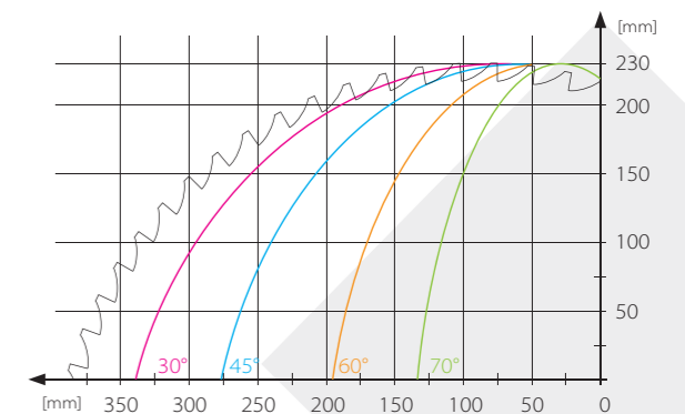
cutting diagram for Crossline 650
