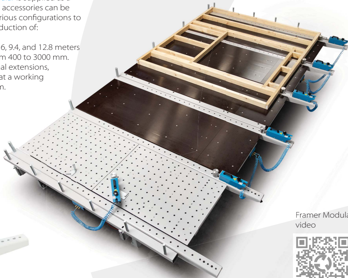
Pneumatic clamps with working force of 1200 N (6 bar)
