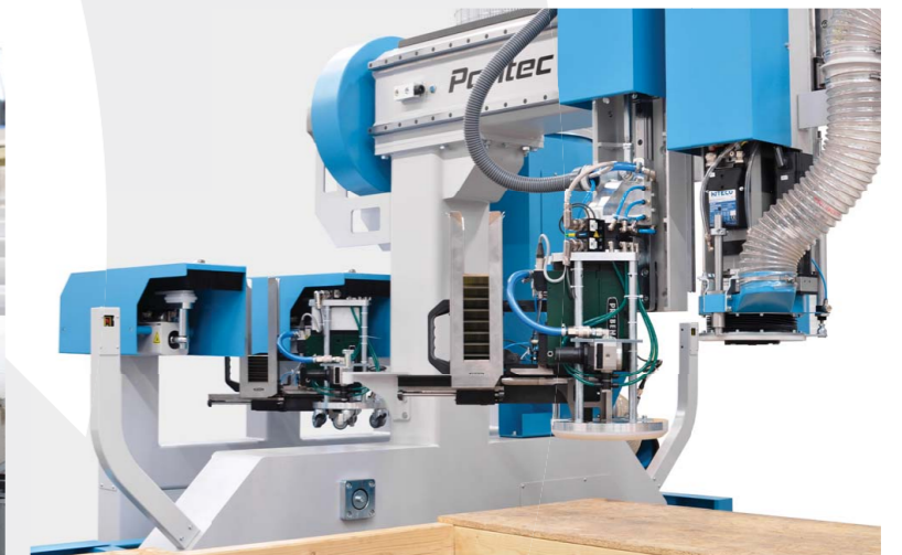
Automatic linear magazine for pneumatic tools
